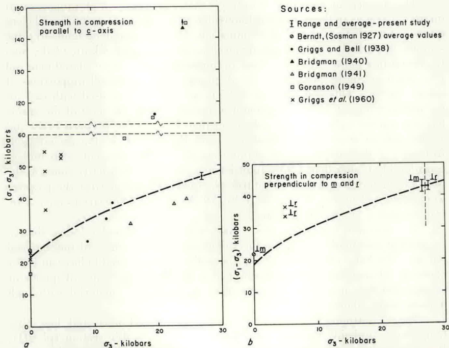
Fig. 9. Strengths of quartz at room temperature and various confining pressures, obtained in the present study and previous studies (as indicated). The broken curves represent strengths predicted by the Griffith theory, using constants derived from the average strengths in the present study.
